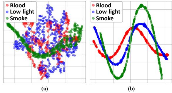
Figure 4: (a) and (b) shows t-SNE visualization between different tasks: (a) Output feature after passing Dual-Domain Prompter; (b) Task Adaptive Embedding output condition.
