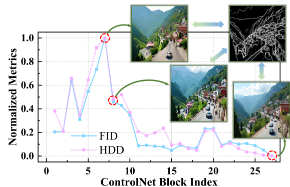
Figure 1: Effect of skipping a specific position within the ControlNet on the quality of the generated image. Higher FID and HDD indicate a more significant impact of the skipped layer on the quality of the final results, reflecting a stronger correlation with the generation.
