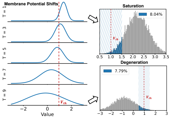
Figure 2: The distribution of membrane potentials deviating from the threshold in a vanilla SNN with ten timesteps. When almost all the membrane potentials of neurons are beyond V_{th} , called saturation. Conversely, called degeneration.
