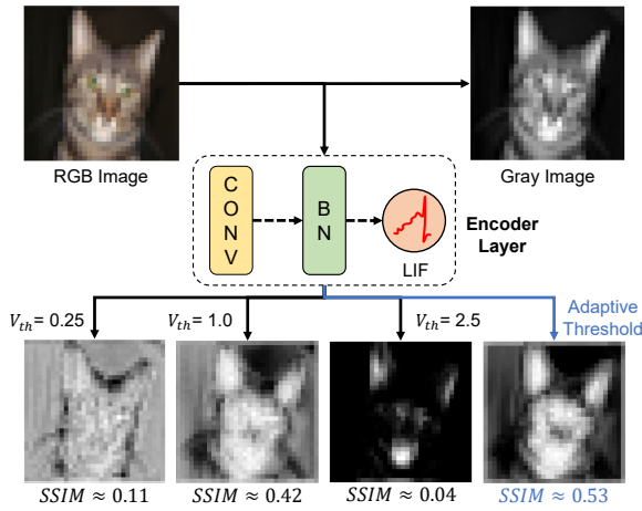
Figure 4: The structural similarity between the gray image and encoded images at different thresholds.
