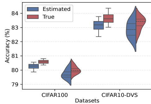
Figure 7: Comparison of estimated with true MPD distribution and w/ vs. w/o moving average (box plot vs. violin plot).
