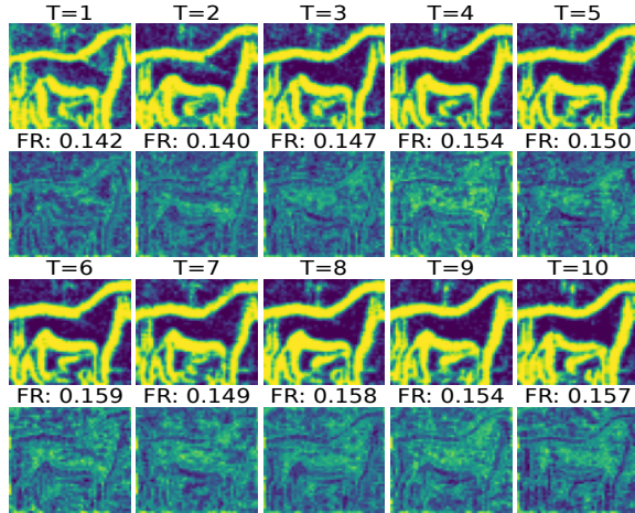
Figure 10: Case study of firing rates (FR) at each timestep.
