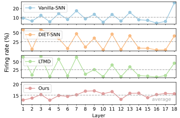
Figure 8: Comparison of firing rates for each layer in ResNet-19, where grey dotted lines denote average values.
