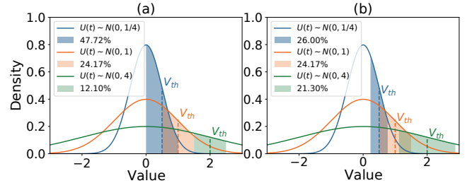
Figure 5: (a) The proportion of membrane potentials that fall into the gradient-available interval with fixed SG ( k = 1 ) under different distributions when using adaptive threshold. (b) The proportion of gradient-available when using the adaptive threshold and threshold-driven gradient optimization.
