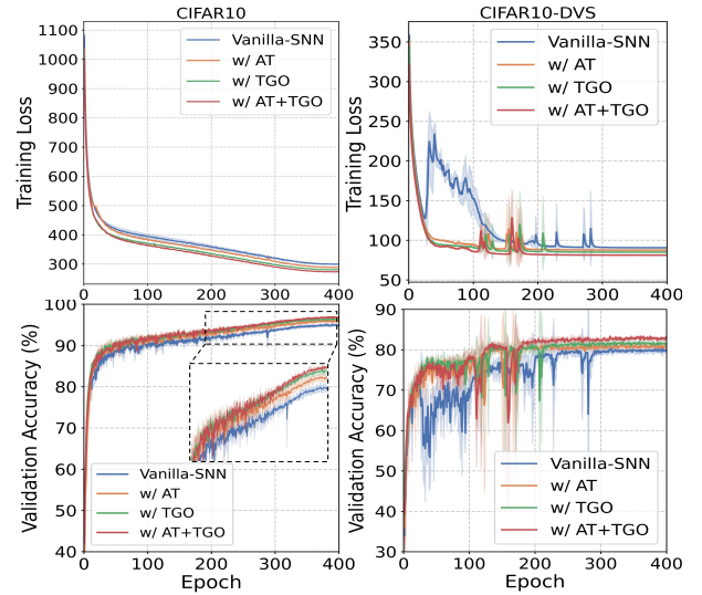
Figure 6: Comparison of training loss and test accuracy.
