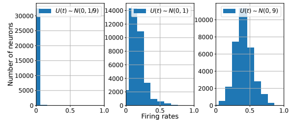
Figure 1: The distributions of firing rates at differ variances of membrane potential when V_{th} = 1.0 (Zheng et al. 2021).
