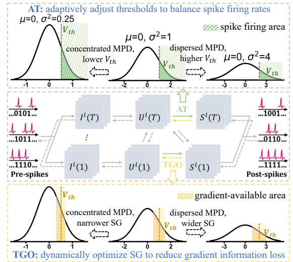
Figure 3: The overall framework of DS-ATGO. Internal dynamics of LIF neurons in a layer (gray). In forward propagation, the adaptive threshold (AT) mechanism promotes neurons to generate stable firing rates under different MPD distributions (green). In backward propagation, the threshold-driven SG optimization (TGO) method dynamically scales SG to respond to evolving MPD (yellow).
