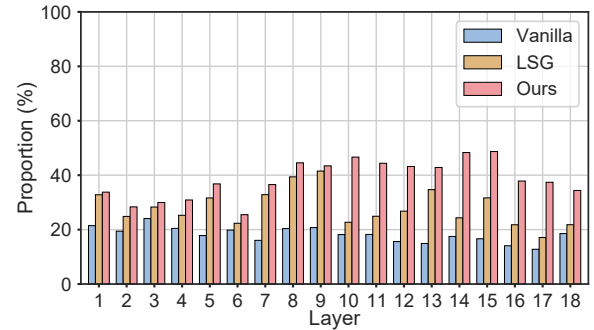
Figure 11: The proportion of neurons falling within the gradient-available interval of each layer in ResNet-19.
