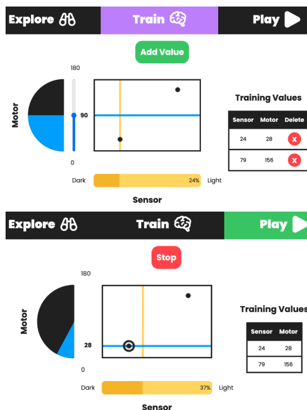
Figure 4: Smart App Train (top): 'Add Value' allows users to add sensor and motor pairs to their training data. Users can also delete data points from the table where the corresponding data point on the graph is highlighted. The yellow vertical line refers to the sensor reading, and the blue horizontal line refers to the angle of the motor in real life. Smart App Play (bottom): After adding all training data, the 'Play' button allows users to test the data. The graph highlights the data point used to inform the algorithm's decision-making.
