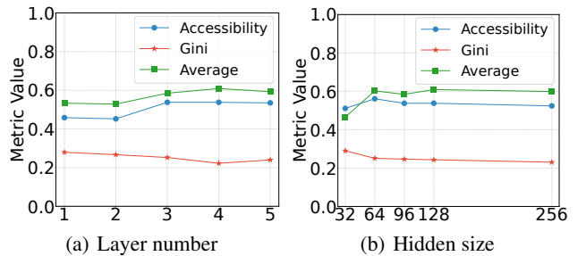
Figure 4: Performance Comparison in the Ablation Study.
