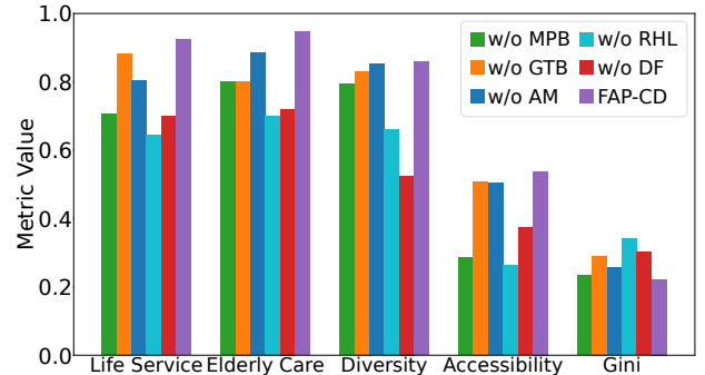
Figure 4: Performance Comparison in the Ablation Study.
