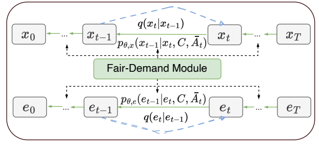
Figure 2: Framework overview of the proposed FAP-CD.
