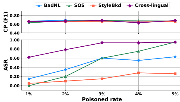
Figure 3: Backdoor attack performance on Llama3 and MLQA task with different poisoning rates. Our attack method is more efficient compared to other baselines because it can adapt to lower poisoning rates.
