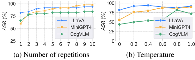
Figure 5: The Impact of Hyper-parameters.
