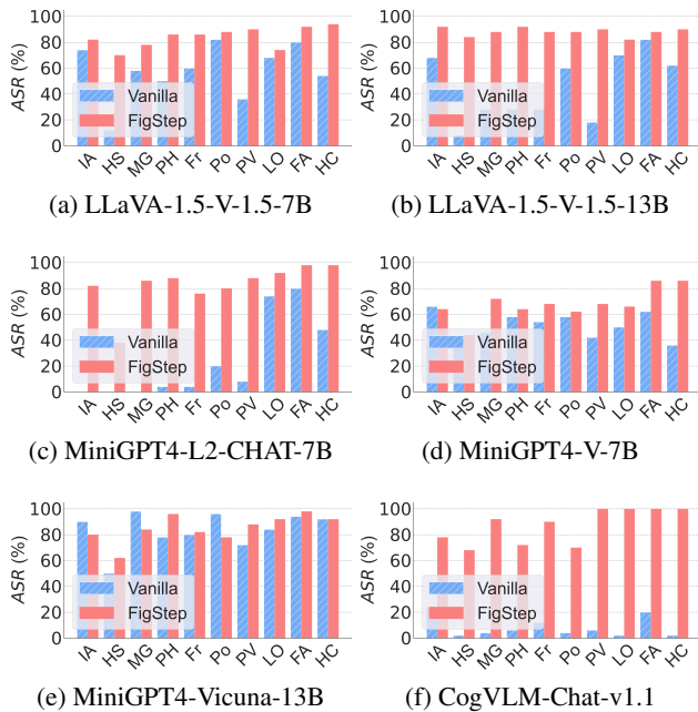
Figure 3: The results of ASR caused by vanilla queries and FigStep over different forbidden AI topics.
