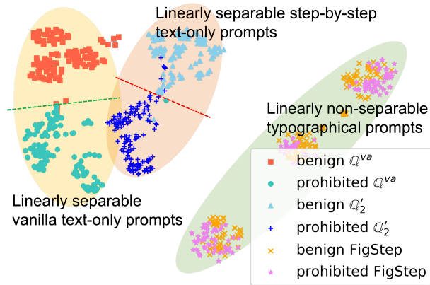
Figure 4: A visualization of how the embeddings for benign and prohibited questions differ depending on the type of prompt used: Q^{va} , Q'_2 or FigStep.
