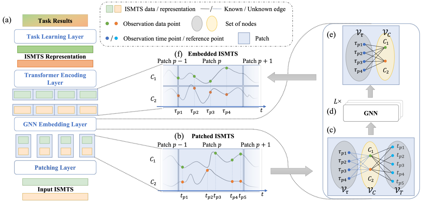
Figure 2: Overview of TimeCHEAT framework, shown in (a), containing 3 main steps, including ISMTS embedding learning , Transformer encoding and task learning . (b) is the patched ISMTS data with p patches. (c) is the initially established bipartite graph with known edges between channel and observation time step nodes and unknown edges between channel and reference point nodes. (d) GNN module for unknown edges learning. (e) Learned edges between channel and reference point nodes. (f) Graph to embedding process to produce embedded ISMTS.
