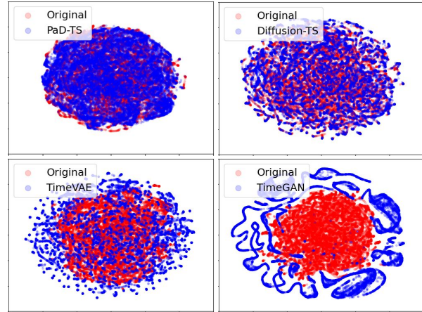
Figure 4: t-SNE plots on the cross-correlation values between original data (red dots) and synthetic data (blue dots) on the Energy dataset.
