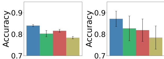
Figure 6: Ablation study on Bitcoin-OTC (left) and Bitcoin-Alpha (right) datasets. Blue:SE-SGformer, Green:SE-SGformer w/o CE , Red:SE-SGformer w/o RE , Yellow:SE-SGformer w/o AE .
