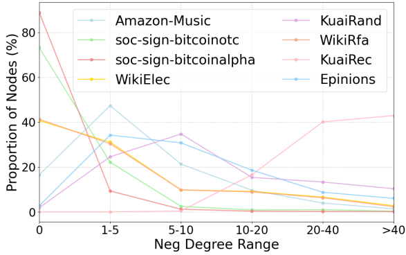
Figure 2: Proportion of node negative degrees and Pos/Neg Ratios across datasets (%)
