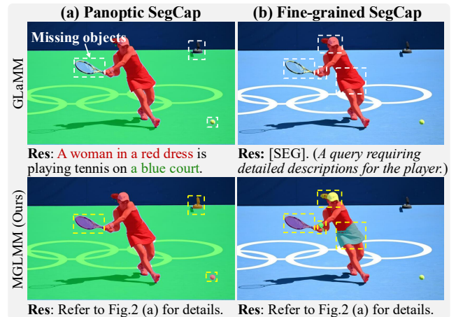
Figure 1: Qualitative comparison between GLaMM and our MGLMM. Please refer to Appendix. A for more details.
