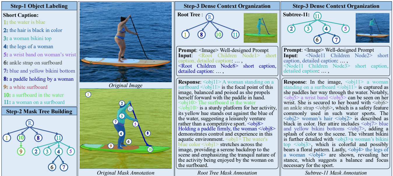
Figure 4: Overview of data auto-annotated pipeline. Best viewed with zoom-in. Please refer to the Appendix. B for more details.
