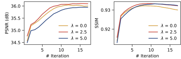
Figure 5: Performance curves of Spener with different \lambda settings on AAPM dataset with 90 views reconstruction under low-dose acquisition.
