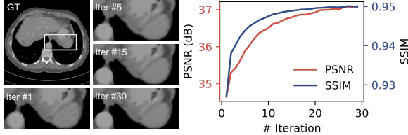
Figure 4: Qualitative results of Spener across different iterations on the AAPM dataset with 90 views.
