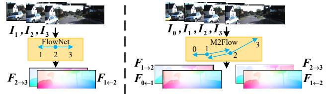
Figure 1: Comparison between previous multi-frame optical flow estimation methods and our approach. (Left) Previous methods assume that the forward and backward flows are equal in magnitude but opposite in direction. (Right) We introduce M2Flow, a novel framework that abandons the constant velocity assumption and integrates multi-frame motion information to concurrently estimate bidirectional optical flows for multiple frames.
