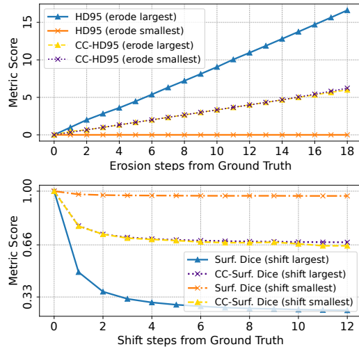
Figure 3: Comparison of the standard Hausdorff95 metric with the CC-Hausdorff95 metric (upper plot), as well as standard Surface Dice with CC-Surface Dice (lower plot). In both scenarios, we start from a perfect prediction and assess the metric scores while degrading the prediction quality of a large versus a small component.
