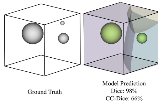
Figure 1: Reporting a Dice of 98% in the shown example, highly overestimates the capability of the trained semantic segmentation model. This might leave radiologists with a false impression of how reliably the model can be used to predict tumors in body scans. With CC-Metrics, we partition an image into distinct regions and evaluate standard semantic segmentation metrics on a per-component basis which gives each tumor the same importance.
