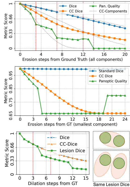
Figure 2: Comparison of Dice, CC-Dice and Panoptic Quality: In the upper plot we start from a perfect prediction and degrade prediction quality by applying erosion to all components uniformly. In the middle plot we only degrade the prediction of the smallest mask. In the lower plot, we compare CC-Dice with Lesion Dice (LD) by using dilation to simulate oversegmentation (left) and highlight a pitfall of LD (right).
