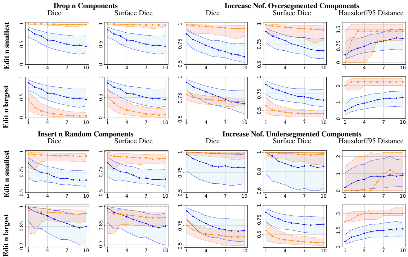
Figure 4: Comparison of standard and CC semantic segmentation metrics on the AutoPET dataset across multiple scenarios. In each graph, the orange line represents the standard metric (e.g., Dice), and the blue line its CC-counterpart (e.g., CC-Dice).
