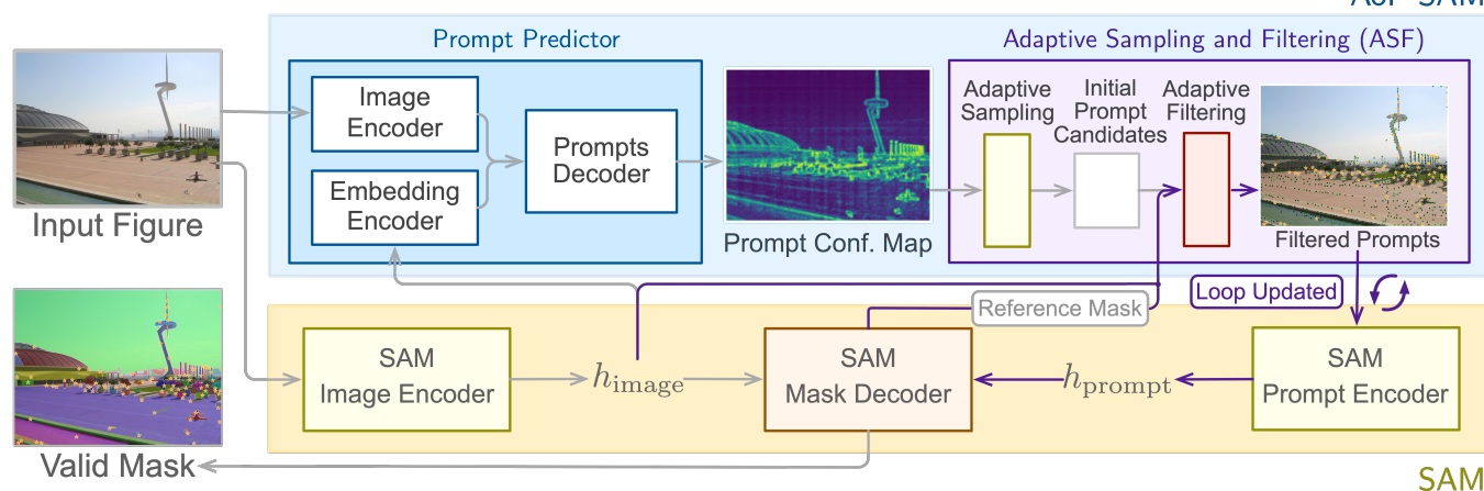
Figure 2: The architecture of our proposed AoP-SAM consists of two key components: the prompt predictor and the Adaptive Sampler and Filter (ASF) Module. The prompt predictor operates by taking the image input and the computed image embedding from SAM’s image encoder as inputs. Prompt predictor then generates a Prompt Confidence Map (PCM) that highlights potential regions for prompt candidates. During test-time, these candidates are adaptively sampled and filtered by ASF, predicting prompts that might lead to redundant masks based on the generated mask references. This process eliminates unnecessary prompts, ensuring that only the essential ones are used to generate the final mask results.
