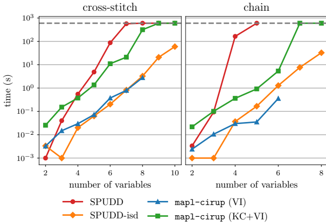
Figure 5: Comparison between mapl-cirup and SPUDD . It reports the value iteration time (VI) and the total time (KC+VI) including the compilation. SPUDD does not distinguish them because it interleaves compilation and VI.
