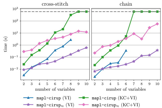
Figure 7: Comparison with and without a linearly approximated utility function. We report the value iteration time (VI) and the total time (KC+VI) including the compilation.
