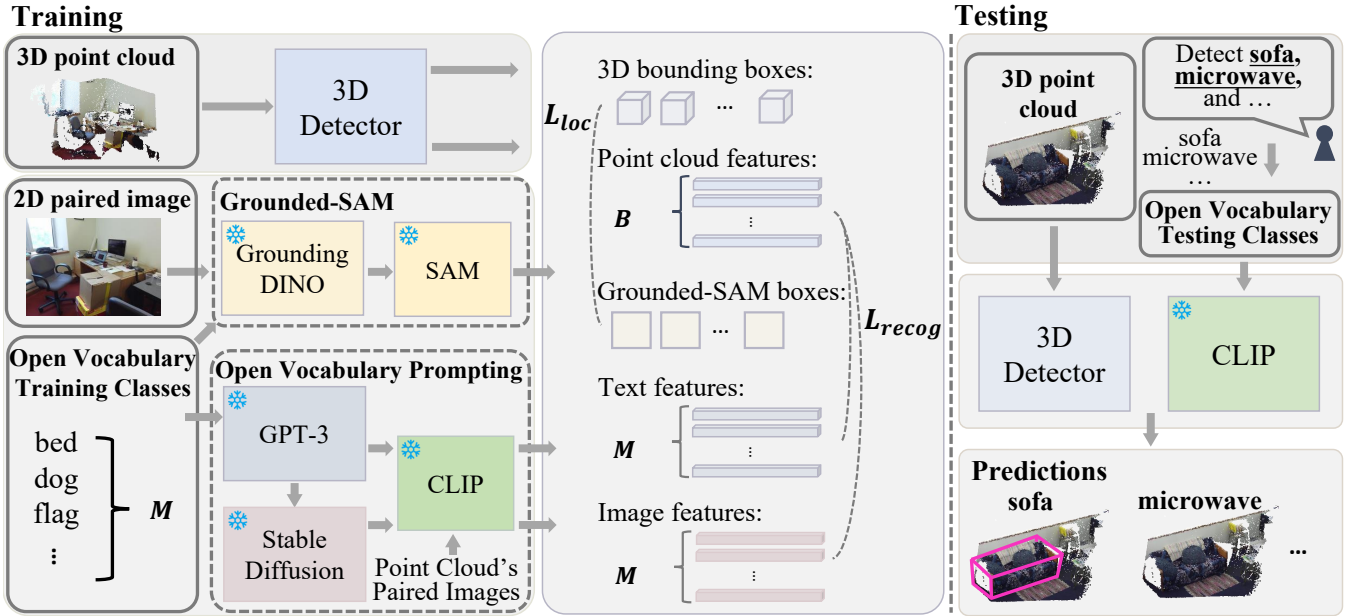
Figure 1: The pipeline of FM-OV3D. Given raw point clouds, corresponding 2D images, and training vocabulary, we train our model leveraging extensive knowledge from pre-trained foundation models, without requiring any annotations. M and B represent the size of the training vocabulary and the number of point cloud samples in a training batch, respectively. L_{loc} aims at improving our 3D detector’s localization ability, while L_{recog} is designed to improve its recognition ability. Point cloud visualization and its paired 2D image are selected from the SUN RGB-D (Song, Lichtenberg, and Xiao 2015) dataset, while training vocabulary is from the LVIS (Gupta, Dollar, and Girshick 2019) dataset. ‘*’ means the model is frozen.
