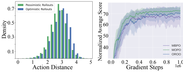
Figure 3: A case study of methods using model MDP (MBPO), P-MDP (MOPO), and O-MDP (OROO) on “Halfcheetah-medium-v2” datasets over 5 different seeds. Left: Histograms of distances between actions from different model rollouts and the offline dataset. Right: Learning curves of different methods.
