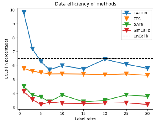
Figure 1: ECEs (%) of CaGCN, ETS, GATS and SimCalib, with different amounts of calibration data. For reference, we also plot the result for uncalibrated backbone as the dashed line.
