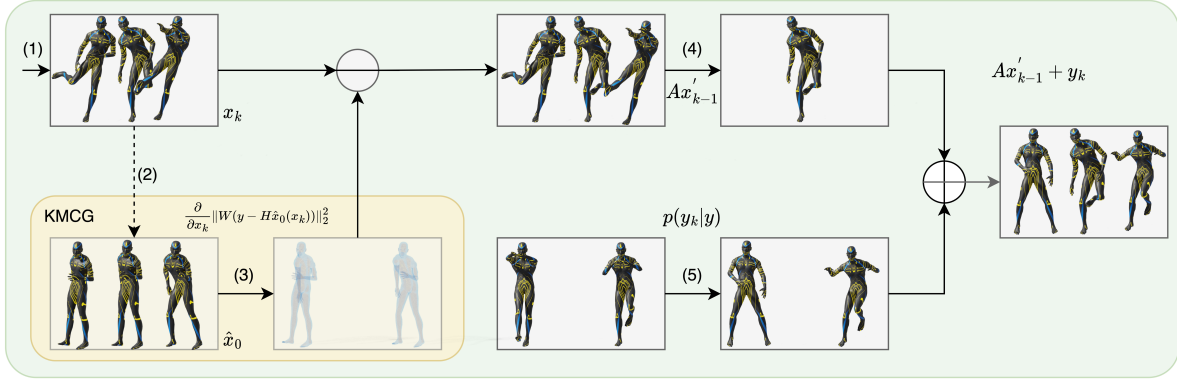
Figure 4: Visual schematic of the Keyframe Manifold Constraint Gradient (KMCGs) correction step. (1) unconditional reverse diffusion generates x_0 . (2) maps the noisy x_k to generate \hat{x}_0 . (3) the manifold constraint gradient \frac{\partial}{\partial x_k} \|W(y - H\hat{x}_0(x_k))\|_2^2 is applied to constraint on the context manifold. (4) Takes the orthogonal complement. (5) Samples from p(y_k|y) , then combines Ax'_{k-1} and y_k to further refine the motion transfer.
