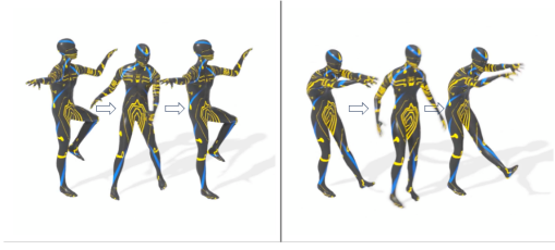
Figure 6: Cycle consistency: Translating the dance motion from the source style to the target style, and then back to the source style. Left: “breaking” to “hip-hop” to “breaking”. Right: “jazz-ballet” to “waacking” to “jazz-ballet”.
