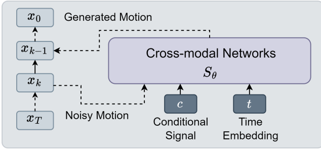
Figure 2: Architecture overview of diffusion models, conditional information acts as cross-attention context. The diffusion model takes noisy sequences and produces the estimated motion sequences.
