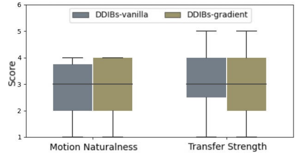
Figure 8: Subjective evaluation results in motion naturalness and transfer strength. Equivalence tests were performed.
