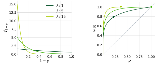
(a) Truncated exponential distributions with rate parameter \lambda \in \{1, 5, 15\} . (b) Utility optimal prices ( \blacktriangledown , \blacktriangledown , \blacktriangledown ) changing as density of patient players concentrates.
