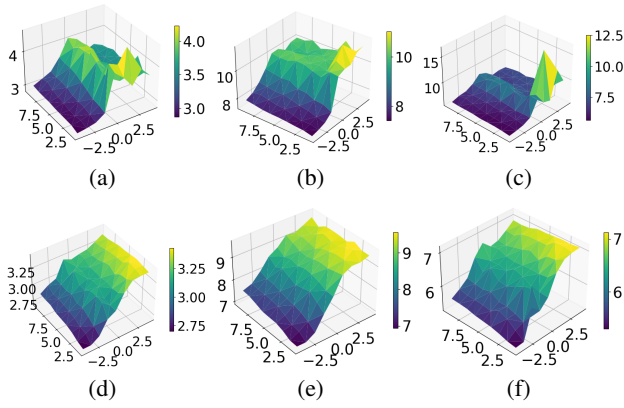
Figure 2: Variation of Individual Metrics under Noise Interference. The x-axis is the noise variance, the y-axis is the noise mean, and z is the individual evaluation index.
