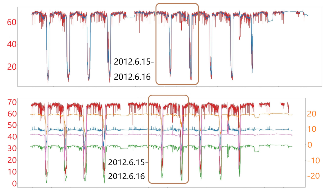
Figure 3: ModWaveMLP 15-min forecasts for node 122 in METR-LA dataset. True value (red), prediction output (a), layer 0 output (b), layer 1 output (green), layer 2 output (orange), and layer 3 output (pink). The y-axis is traffic speed (mph), and the x-axis is the date (2012.6.8-2012.6.21).
