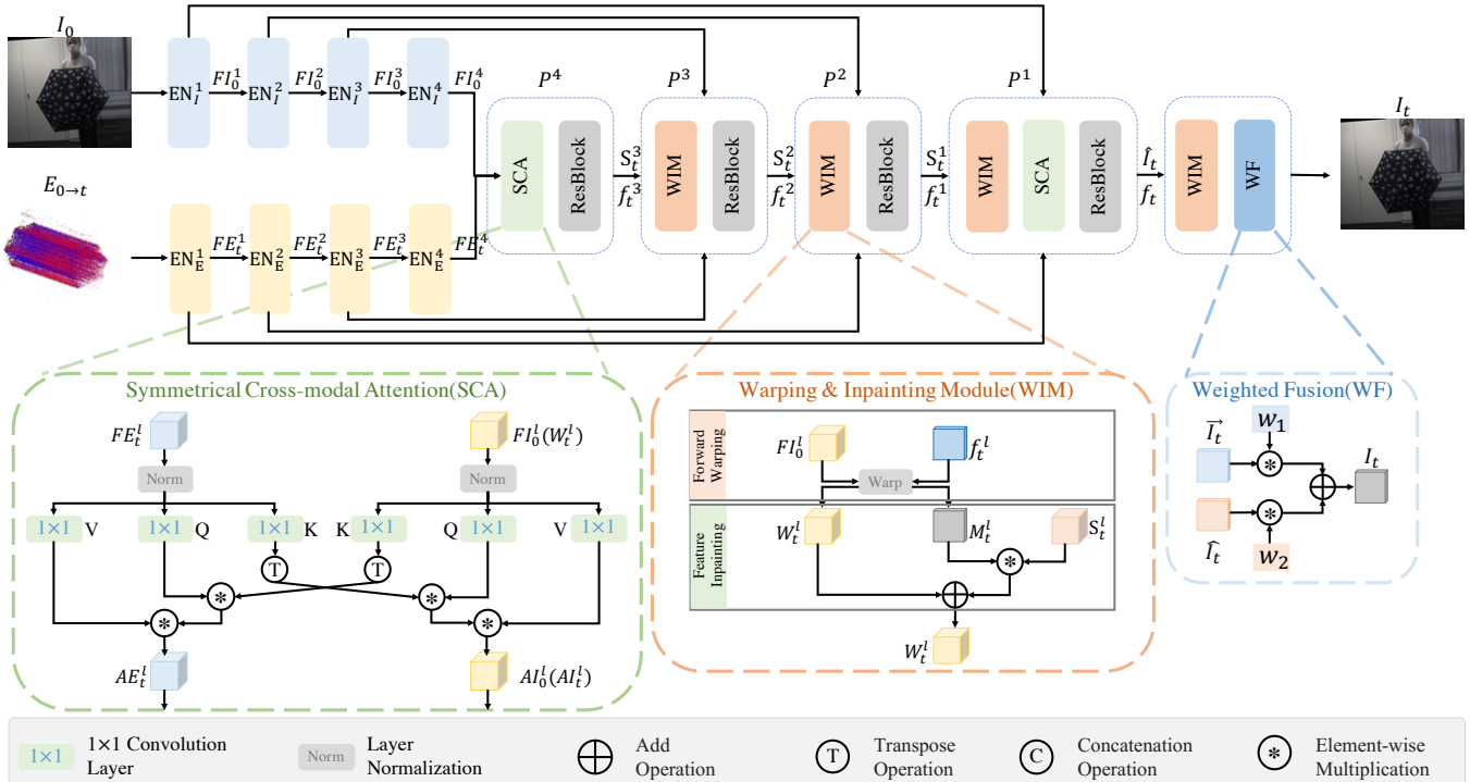
Figure 2: Overview of our proposed network model. In our framework, we first use two encoders to extract pyramid features for the image and events. Then we apply a coarse-to-fine joint decoder to get the synthesized feature and optical flow at each pyramid layer. In the decoder, we utilize Symmetrical Cross-modal Attention to augment both image and event features. We also introduce Warming and Inpainting Module to repair the holes caused by forward warping and get spatially-aligned image features. Finally, we adopt Weighted Fusion to output the final frame prediction from the synthesized and warped frames.
