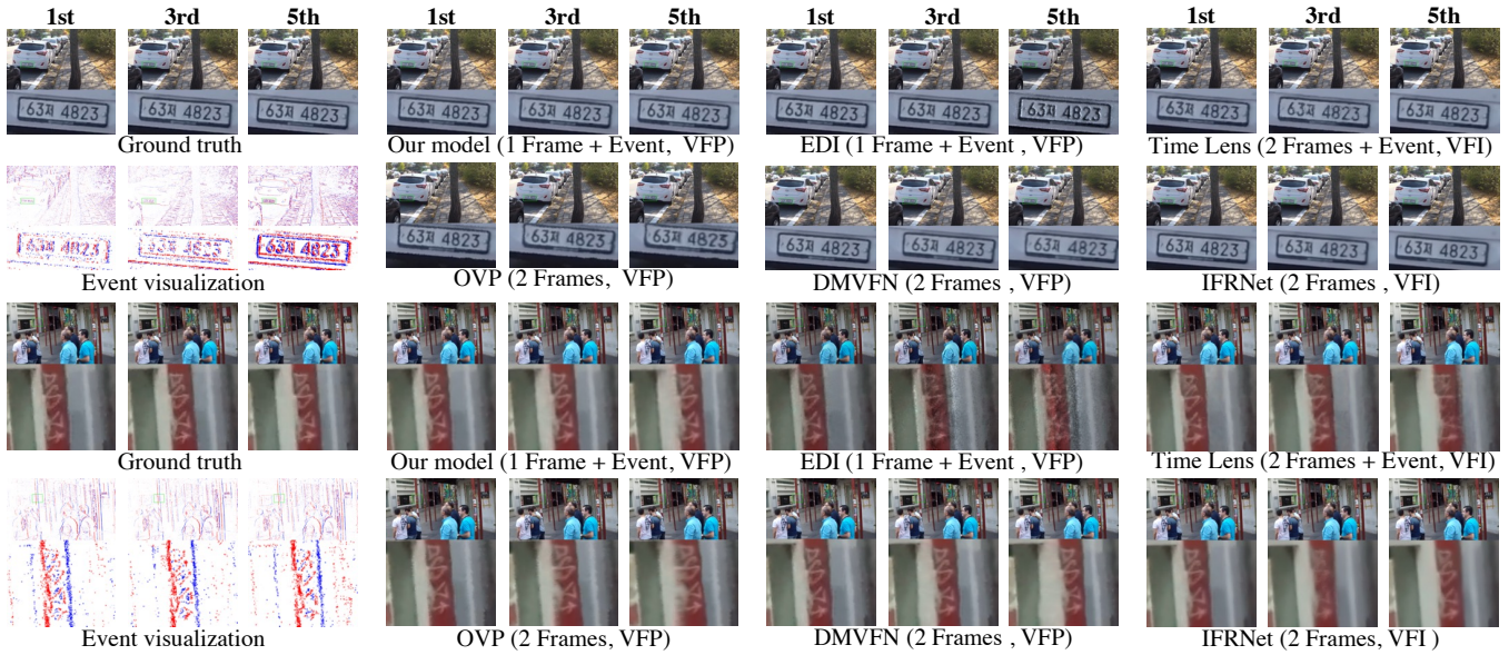
Figure 4: Visual comparisons on the GoPro dataset with synthetic events.
