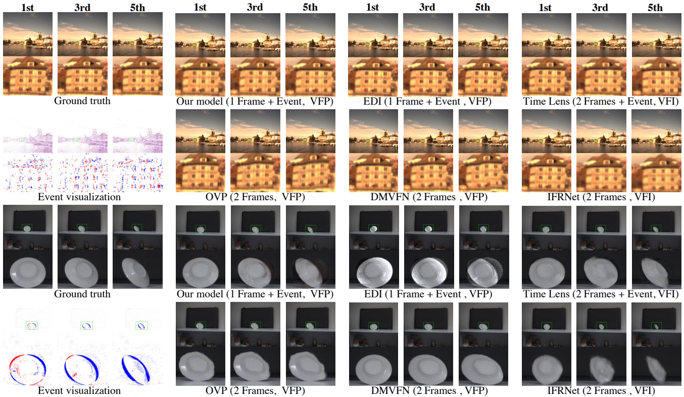
Figure 5: Visual comparisons on the real-captured HS-ERGB dataset.
