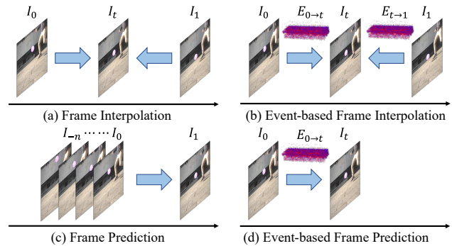
Figure 1: Differences between VFI, event-based VFI, VFP and event-based VFP. VFI methods require the image (and events) after the target time t , while image-based VFP is subject to the limited complexity of motion expressed in fixed frame rate inputs. Event-based VFP can solve the above problems, and this paper focuses on the minimal setup of combining a single frame with the following events.
