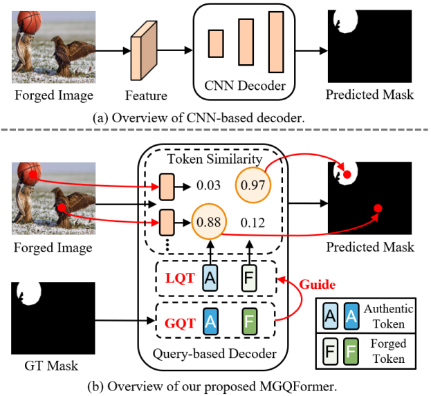
Figure 1: The difference between previous methods and ours. Our method uses a query-based transformer which is efficient and explainable. Token similarity means the softmax result of the scalar product between the image feature and query tokens. In addition, we use ground-truth masks to guide the learnable query token (LQT) in identifying the authentic and forged regions.
