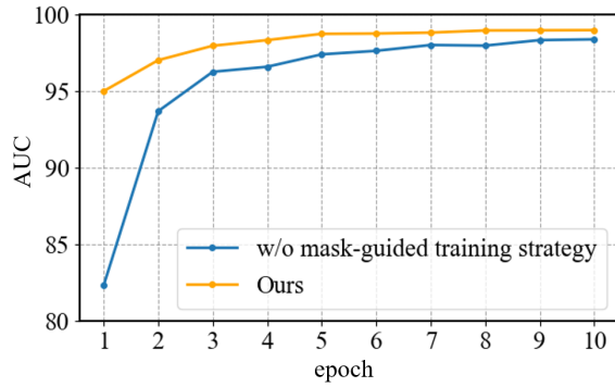
Figure 3: AUC scores (%) of MGQFormer without and with mask-guided training on the validation split of the synthesized dataset in different training epochs.
