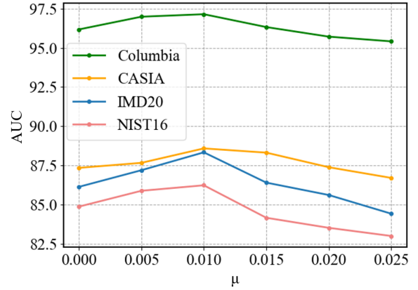
Figure 4: The effect of parameter \mu in mask-guided training.
