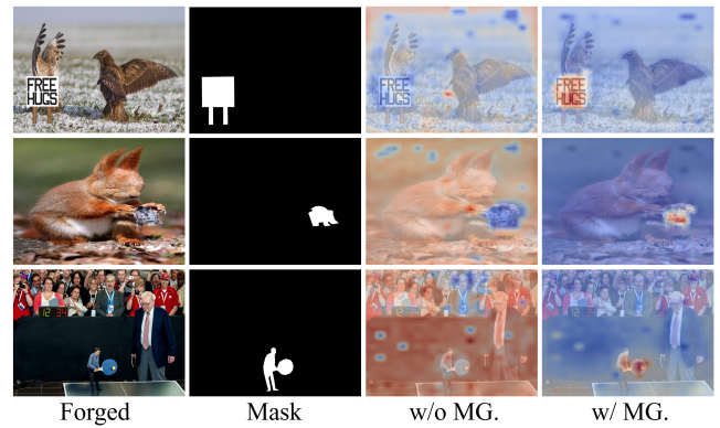
Figure 7: Visualization of attention maps for the proposed mask-guided training. From left to right, we display the forged images, GT masks, and attention maps for LQT representing the forgery in Transformer decoder without (w/o) and with (w/) mask-guided training, respectively.
