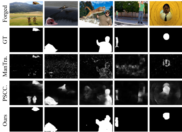
Figure 5: Visualization of the predicted manipulation mask by different methods. From top to bottom, we show forged images, GT masks, predictions of ManTraNet, PSCC-Net, and ours.
