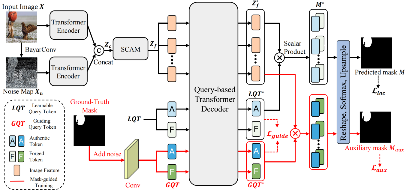
Figure 2: An overview of the proposed framework MGQFormer consisting of two-branch transformer encoder, a fusing module, and a mask-guided transformer decoder. During training, the input is a suspicious image ( H \times W \times 3 ) and a ground-truth mask, the output includes a predicted mask and an auxiliary mask ( H \times W \times 1 ) which are both involved in loss computation ( \mathcal{L}_{loc} and \mathcal{L}_{aux} ). Note that the red-line part is mask-guided training and is not required during inference.
