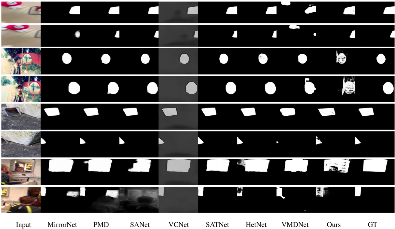
Figure 8: Visual comparison between ZOOM (weakly-supervised) and existing mirror detectors (fully-supervised).
