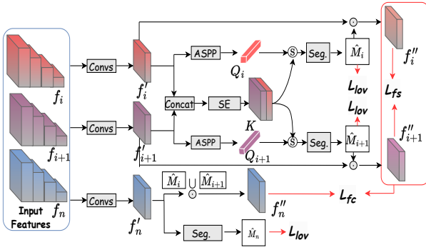
Figure 7: Proposed temporal similarity-contrast modeling module. It aims to enhance feature similarity between mirror regions in adjacent frames and maximize feature contrast between mirror/non-mirror regions in distant frames.
