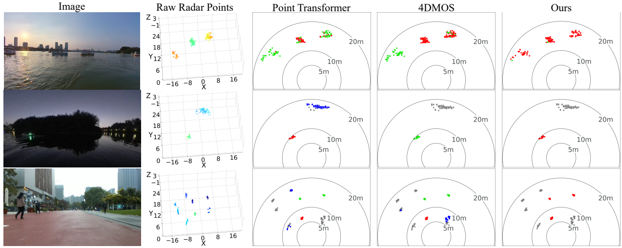
Figure 4: Qualitative results of PT, 4DMOS and ours. Red points are the true moving points, gray points are the true static points, green points are the false moving points, and blue points are the false static points. Better view with colors.
