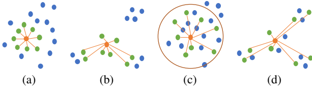
Figure 2: The orange point is the source point, the green points are the points sampled by the source point and the blue points are the other points. (a) is the sampling result if k is small, (b) is the sampling result if k is large, (c) is the sampling strategy of Object Attention and (d) is the sampling strategy for Scenario Attention.
