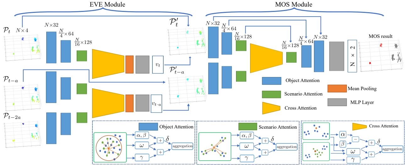
Figure 3: MOS-EVE network for ego-velocity estimation(EVE) and moving object segmentation(MOS module)
