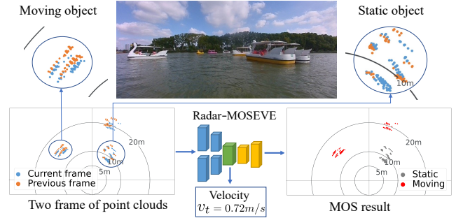
Figure 1: Our MOSEVE network takes two frames of radar point clouds as input and outputs the current ego velocity of the robot. The MOS module takes the velocity-calibrated point clouds to provide the moving segmentation.
