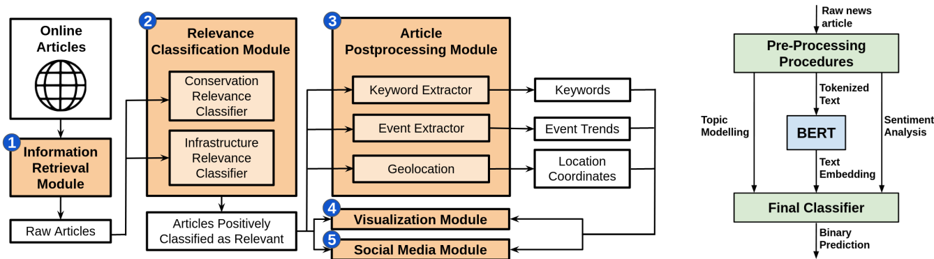
(a) Diagram of overall NEWSPANDA pipeline, with the five key modules in orange boxes. Generated outputs of NEWSPANDA are in the white boxes.
