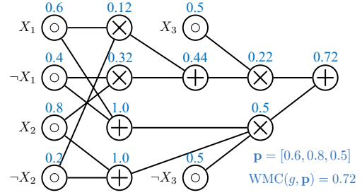
Figure 3: An example decomposable and deterministic LC g representing X_3 \Leftarrow (X_1 \wedge \neg X_2) \vee (\neg X_1 \wedge X_2) . WMC of g w.r.t. \mathbf{p} = [0.6, 0.8, 0.5] is labeled blue beside each node.
