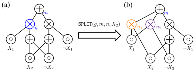
Figure 4: An example of the SPLIT operation.
