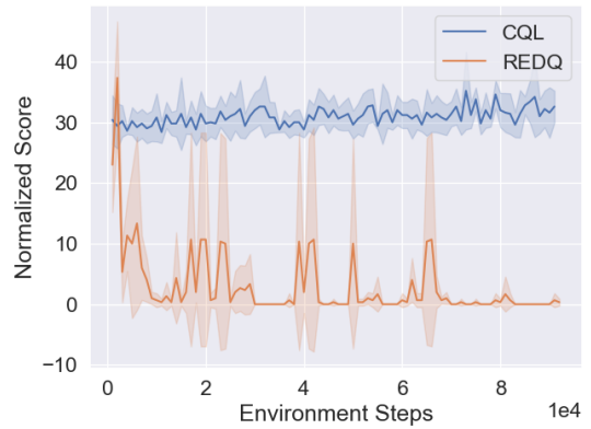
Figure 1: Learning curves for the online agent initialized with the D4RL (Fu et al. 2020) dataset hopper-medium-replay-v0. Scores are averaged over five random seeds and the shaded areas represent the standard deviation. The normalized score of 100 is the average returns of a domain-specific expert while normalized score of 0 corresponds to the average returns of an agent taking uniformly random actions across the action space.
