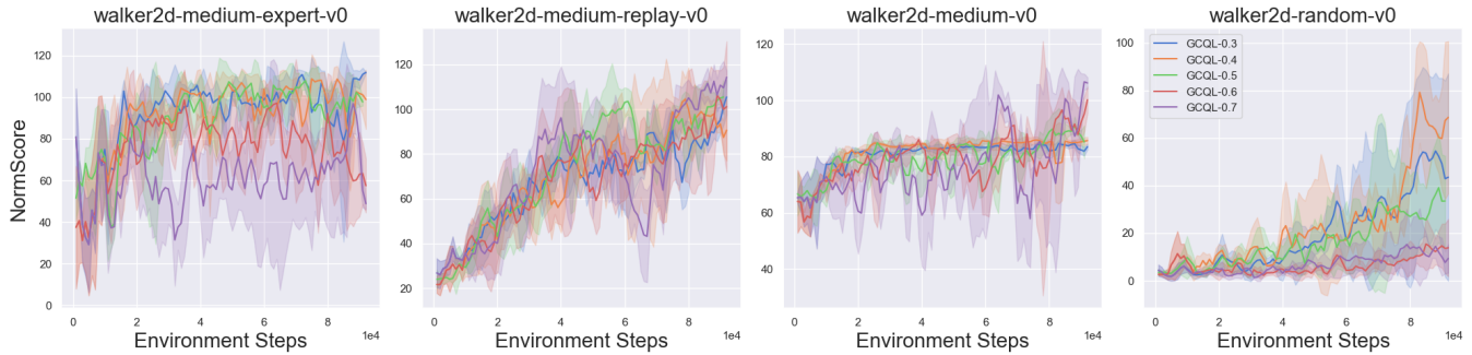
Figure 4: Learning curves for agents with different OORB threshold p . GCQL- X means that p is set to X . Results are averaged over three random seeds.
