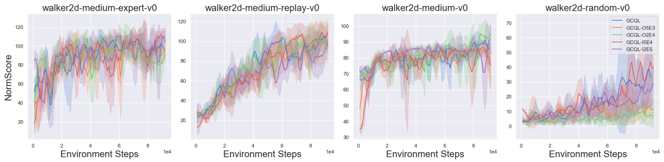
Figure 3: GCQL-i2e5 and GCQL-i5e4 mean that T_{\text{initial}} is 2e5 and 5e4 , respectively. And GCQL-o2e4 and GCQL-o5e3 mean T_{\text{off}} is set to corresponding values. Results are averaged over three random seeds.
