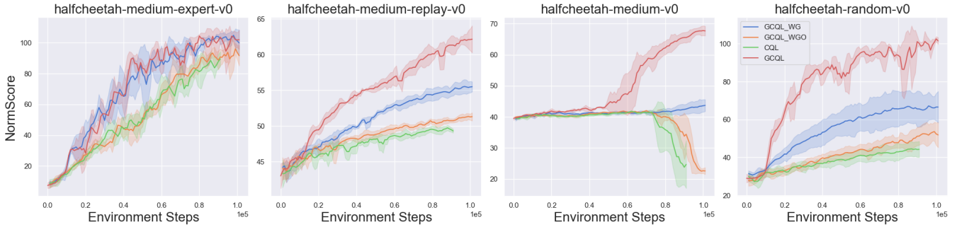
Figure 2: Ablation studies on Halfcheetah. GCQL_WG: GCQL without the greedy updating strategy. GCQL_WGO: GCQL without the greedy updating strategy and online buffer. Results on four tasks are averaged over three random seeds.
