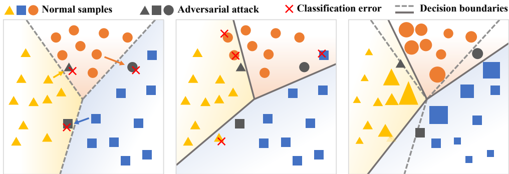
Figure 3: Left panel: Decision boundary of plainly trained model. Middle panel: Decision boundary of AT-trained model. Right panel: Decision boundary of DBFAT-trained model. We use the dotted line to represent the boundary of the clean model, and solid line to represent the boundary of the robust model. The size of the shape represents the value of the weight. Those samples that are close to/far from boundary are assigned larger/smaller weight. The decision boundary of DBFAT-trained model (see the right sub-figure) can achieve a higher A_{rob} and meanwhile maintain A_{cln} .
