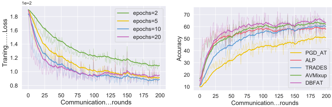
Figure 4: Left: Convergence rate for different local epochs. Right: Accuracy of FedAvg combined with different AT methods.
