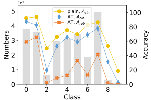
Figure 2: Test accuracy on a randomly selected client.
