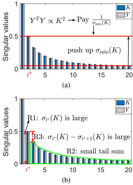
Figure 2: (a) We use the square root of \mathcal{P}_{i^*}(\mathbf{Y}^T \mathbf{Y}) to approximate K so that we pay a factor of 1/\sigma_{i^*}(K) , instead of 1/\sigma_{\min}(K) . (b) Three key requirements for i^* : • (R1) \sigma_{i^*}(K) is large, • (R2) \mathcal{P}_{i^*}(K^2) is close to K^2 , and • (R3) \sigma_{i^*}(K) - \sigma_{i^*+1}(K) is large.
