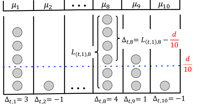
Figure 3: A toy example of nparam-gEST when K_{i,j} = 1 for all i and j and \Omega = [-1, 1] and is uniformly partitioned into 10 pieces. Sampling a g(\mathbf{x}_{t,i}) corresponds to randomly placing a ball into a total number of 10 bins. For example, \mathbf{x}_{t,2} falls into the 8-th interval so \mu_8 is used to approximate g(\mathbf{x}_{t,2}) , which may be viewed as a new ball of type \mu_8 (or in 8-th bin) is created. The mean load for each bin is d/\ell = d/10 . We calculate \sum_{i \leq d} g(\mathbf{x}_{t,i}) by counting the balls in each bin: \mathbf{y}_{t,1} = 5 \times \mu_1 + 1 \times \mu_2 + \dots + 6 \times \mu_8 + 3 \times \mu_9 + 1 \times \mu_{10} + \xi_{t,1} .
