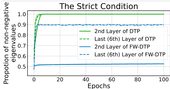
(b) Positive semi-definiteness of J_{f_i} J_{g_i}
