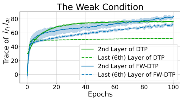
(a) Trace of J_{f_i} J_{g_i}
