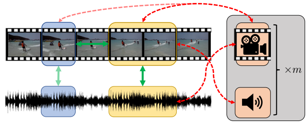
Figure 1: Illustration of Contrastive Loss Terms in our Model. We demonstrate the main contrastive pairs in our formulation given an example video clip (yellow box in the middle) and its corresponding audio clip. Positives (solid green arrows) are constructed from differently augmented video clips of the same training instance (blue box) and temporally aligned pairs of the corresponding video and audio clips. Negatives (dashed red arrows) stem from m other video and audio clips from the current mini-batch or a memory bank of prior embeddings (gray box on the right). Additional positives from the memory bank are omitted from the figure. Note that our formulation does not contain any contrastive terms among audio clips.
