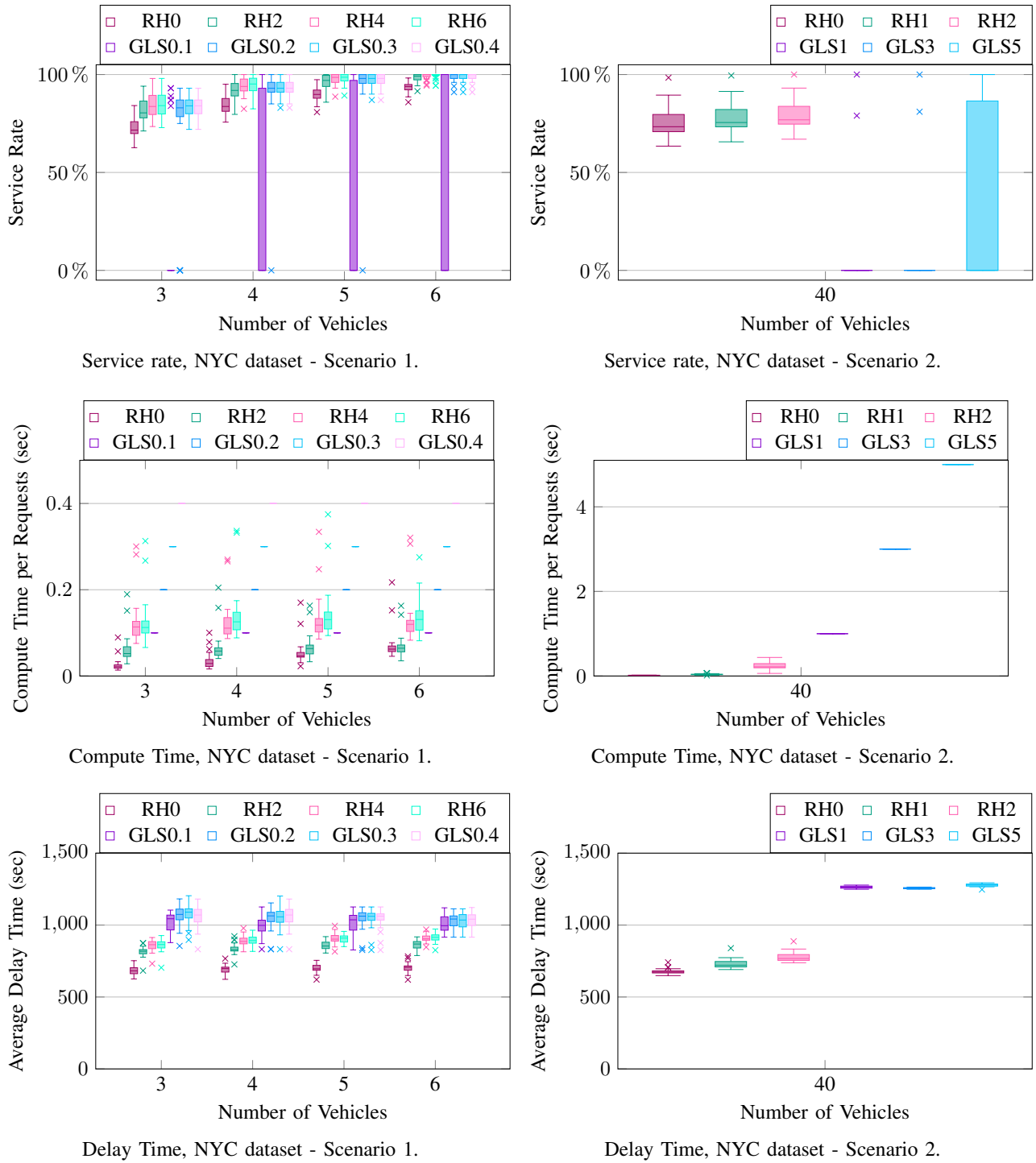
Figure 3: Comparison of the rolling horizon framework with the baseline approach. RH X denotes the rolling horizon solutions with X indicating the rolling horizon factor. GLS Y denotes the guided local search solutions with the Y indicating time limit.
