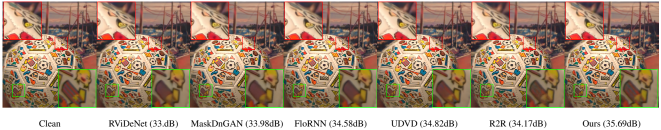
Figure 2: Real raw denoising on CVPD dataset. All raw data has been transferred to RGB domain for visualization. Our method requires no external clean videos for training opposite to supervised methods..
