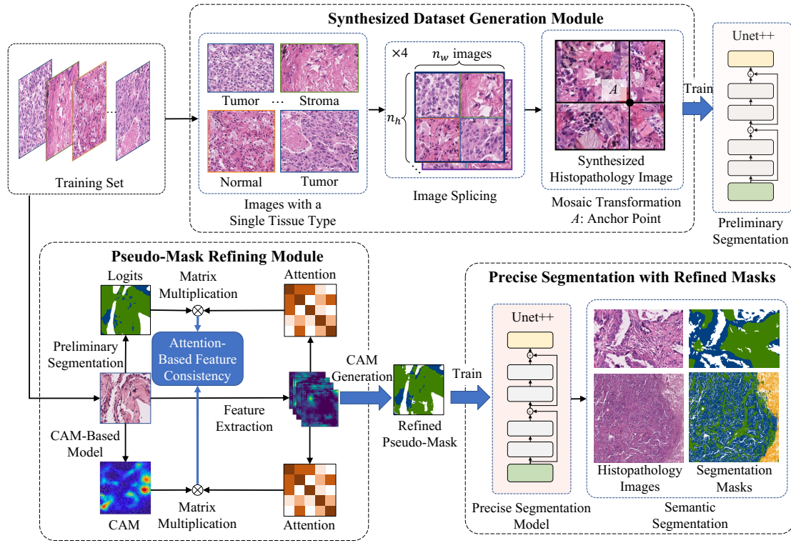
Figure 2: An overview of the PistoSeg framework. Firstly, based on the Mosaic transformation, a synthesized dataset generation module generates synthesized histopathology images with pixel-level masks, which are utilized to train a preliminary segmentation model. Next, assisting with an attention-based feature consistency, a pseudo-mask refining module generates refined masks, which are utilized to train a precise segmentation model for semantic segmentation with higher accuracy.
