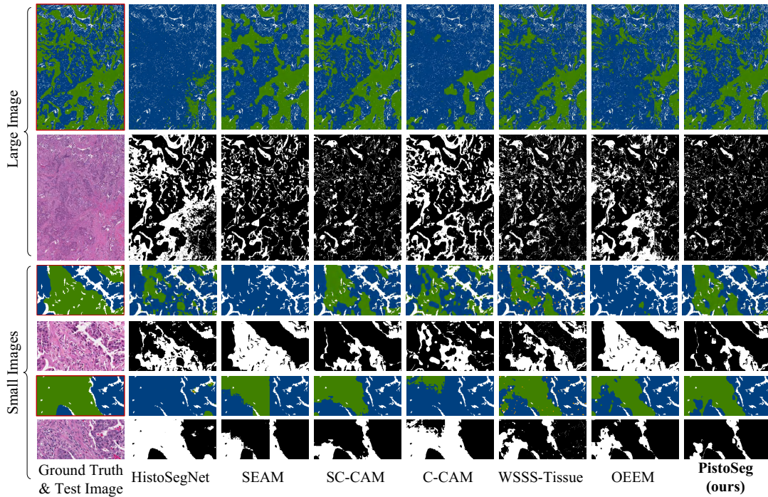
Figure 3: Visualization of segmentation masks on the WSSS4LUAD test dataset of PistoSeg and comparison methods. Blue, green, and yellow represent tumor, stroma, and normal tissue. The black and white masks represent the differences between the ground truth and the predicted mask. Black stands for the same label and white represents difference. Ground truth masks are denoted with red borders.
