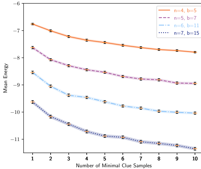
Figure 6: Energy decreases as the number of sampled minimal clue sets increases.
