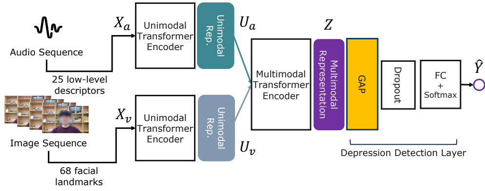
Figure 3: An illustration of the proposed model, Depression Detector .
