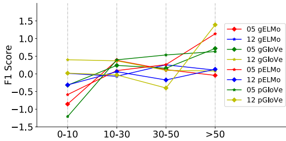
Figure 2: Relative improvements of our second-order model over our first-order model on sentences of different lengths. g and p in the legend represent the settings of gold predicates and predicted predicates respectively.
