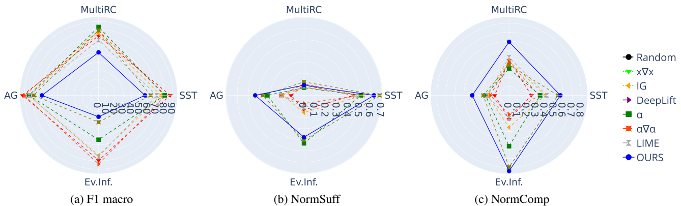
Figure 1: F1 macro (lower is better), mean NormSuff (higher is better) and mean NormComp (higher is better), when using any single feature scoring method across all instances in a dataset and our proposed method of selecting a feature scoring method for each instance (OURS) for TOPK rationale types.
