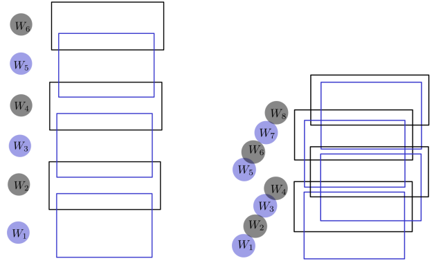
(a) Alternating regions for an edge. (b) Regions for an edge with shift, when \Delta = 4 . Each region W_i starts at same horizontal position as W_{i-4} .
