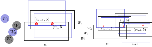
(a) Edge e_i appearing at time 5 and the corresponding placement of vertex appearances to vertex appearances placement in the rectangles, when \Delta = 4 . (b) Edges e_i and e_{i+1} appearing at time 5 and the corresponding placement of vertex appearances to vertex appearances placement in the rectangles, when \Delta = 4 .
