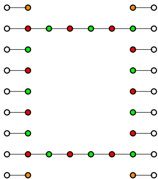
Figure 2: An example of two optimum covers (red and green) of a segment block, where the orange vertices are always included in the solution.
