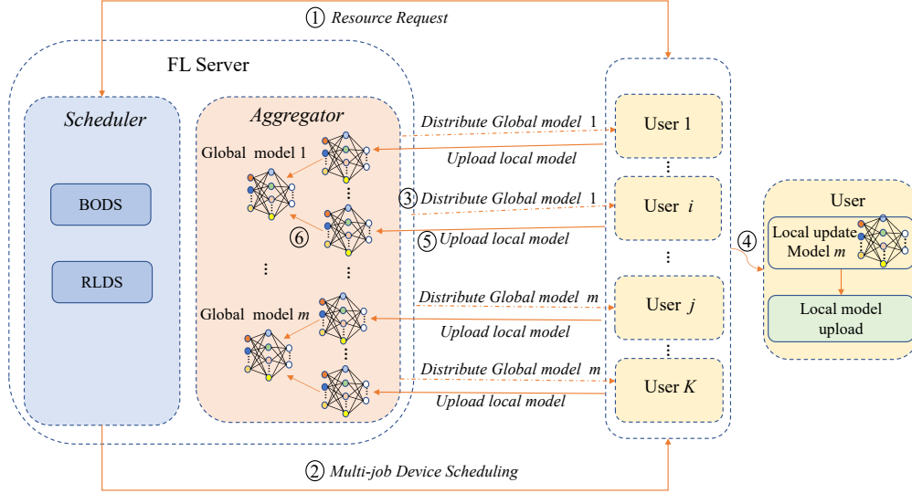
Figure 1: The training process within the Multi-job Federated Learning Framework.
