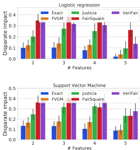
Figure 4: Comparing the average accuracy of different verifiers over 100 synthetic benchmarks while varying the number of features. FVGM yields the closest estimation of the analytically calculated Exact values of DI for LR and SVM classifiers.
