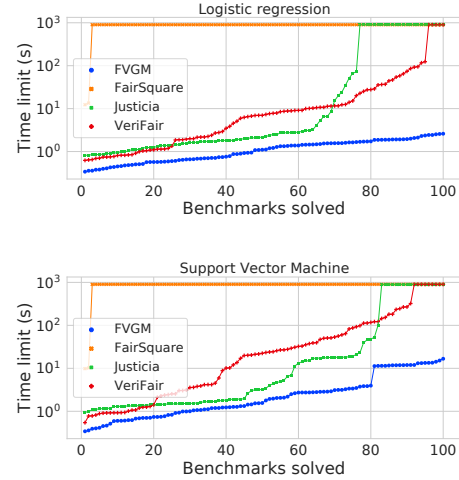
Figure 3: A cactus plot to present the scalability of different fairness verifiers. The number of solved benchmarks are on the X-axis and the required time is on the Y-axis; a point (x, y) implies that a verifier takes less than or equal to y seconds to compute fairness metrics of x many benchmarks. We consider 100 benchmarks generated from 5 real-world datasets using 5-fold cross-validation. In each fold, we consider \{25, 50, 75, 100\} percent of non-sensitive features.
