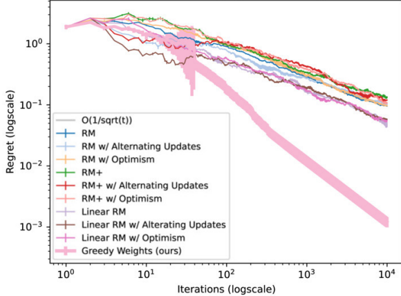
(a) Regret v. Iteration
