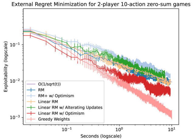
(b) Exploitability v. Time
