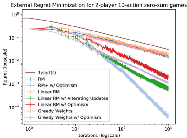
Figure 2: In the special case of two-player zero-sum games where mixed strategies are used at each iteration is applied, greedy weights (combined with optimism (Syrngkanis et al. 2015)) outperforms many but not all previous methods for minimizing external regret. However, this trick is not feasible for general computation of equilibria or in games with a large number actions where full queries to the payoff matrix are too expensive.
