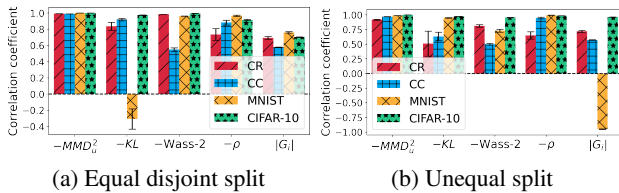
Figure 2: Correlation of (negative of) metrics and |G_i| with \alpha_i (higher is better).
