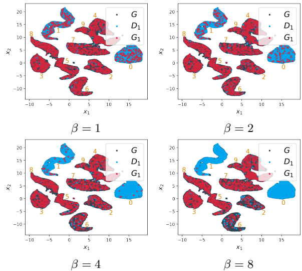
Figure 1: Synthetic data points G_1 (visualized in 2-D embedding using UMAP (McInnes, Healy, and Melville 2018)) as reward to party 1 with varying \beta in equal disjoint split. Each cluster has majority of the MNIST digit in yellow.
