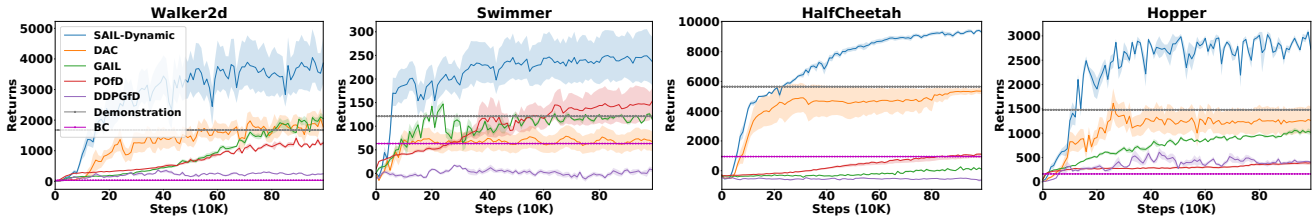
Figure 2: Learning curves of SAIL and other baselines using 1 suboptimal demonstration trajectory.
