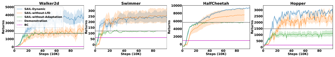
Figure 4: Ablation study by removing different algorithmic components from SAIL , given one teacher trajectory.
