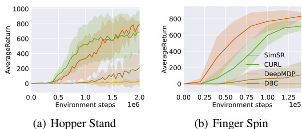
Figure 3: Performance comparisons on 2 DMC tasks over 5 seeds with one standard error shaded in the natural video setting.
