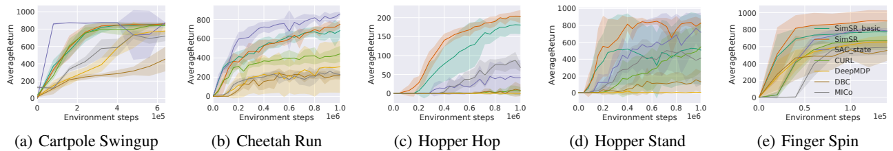
Figure 1: Performance comparison on 5 DMC tasks over 5 seeds with one standard error shaded in the default setting. For each seed, the average return is computed every 10,000 training steps, averaging over 10 episodes. The horizontal axis indicates the number of environment steps. The vertical axis indicates the average return.
