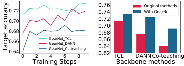
Figure 2: Universal capability of GearNet on D \rightarrow W with Unif-20% noise under WSDA (TCL), de-noise (Co-teaching) and UDA (DANN) backbone methods. (a) Trend of target accuracy across training steps. (b) Best target accuracy across training steps
