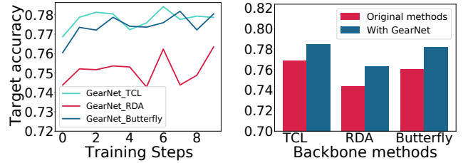
Figure 3: Universal capability of GearNet on W \rightarrow D with Unif-20% noise for three different WSDA (TCL, RDA, Butterfly) backbone methods. (a) Trend of target accuracy across training steps. (b) Best target accuracy across training steps.
