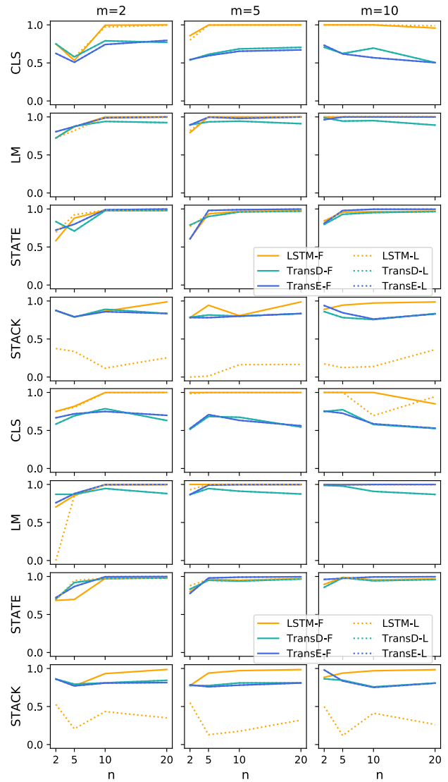
Figure 15: Performance on (wcv^r)^n . Top 4 rows show k = 3 , and the lower 4 rows show results with k = 5 .
