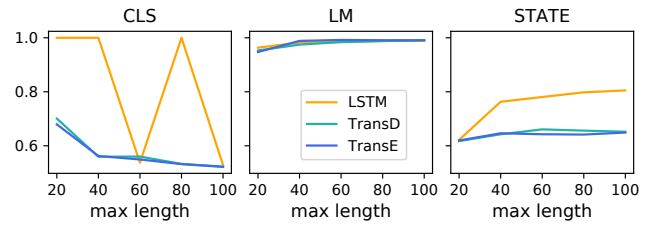
Figure 8: Performance on parity
