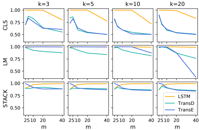
Figure 7: Performance on Dyck.
