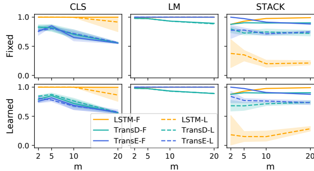
Figure 17: Model performance on Dyck-(5,*). First row shows results with Equation (5), and second row shows results with Equation (6). Lines indicate the average accuracy over 5 runs, and the shadows illustrate the range.
