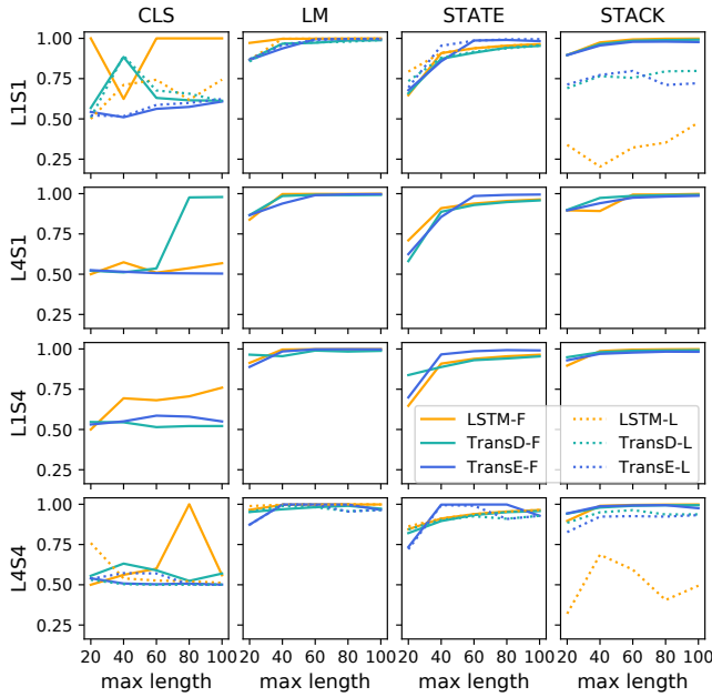
Figure 16: Performance on a^n b^n . Y-label shows number of layers and scaling factor \alpha . For example, L1S4 represents single-layer model with \alpha = 4 .
