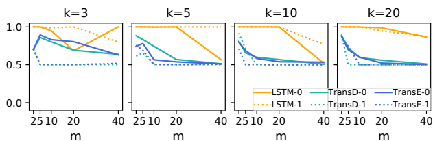
Figure 23: Two-phase classification accuracy on Dyck.
