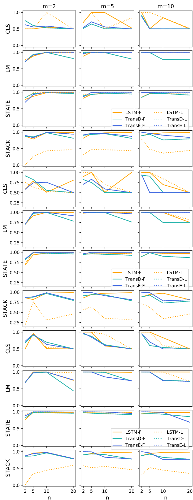
Figure 20: 4-layer model with \alpha = 4 on (wcv^n)^n . Upper 4 rows: k = 3 ; middle 4 rows: k = 5 ; bottom 4 rows: k = 10 .
