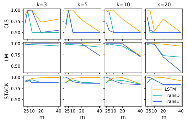
Figure 18: Performance on Dyck ( \alpha = 1 , four layers)
