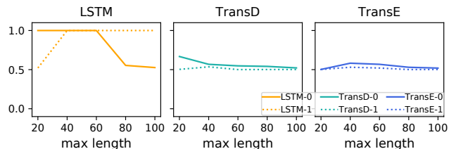
Figure 22: Two-phase classification accuracy on parity.
