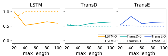
Figure 21: Two-phase classification accuracy on a^n b^n .
