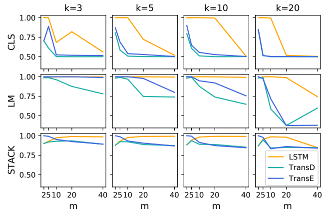
Figure 19: Performance on Dyck ( \alpha = 4 , single layer)
