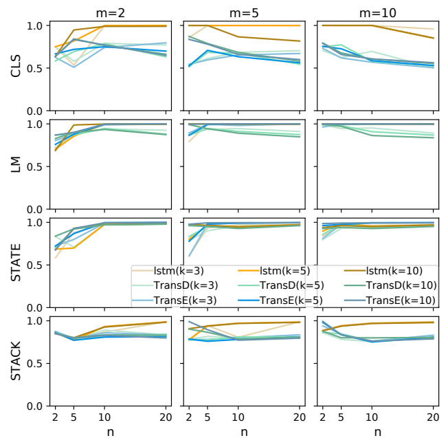
Figure 9: Performance on (wcv^r)^n .
