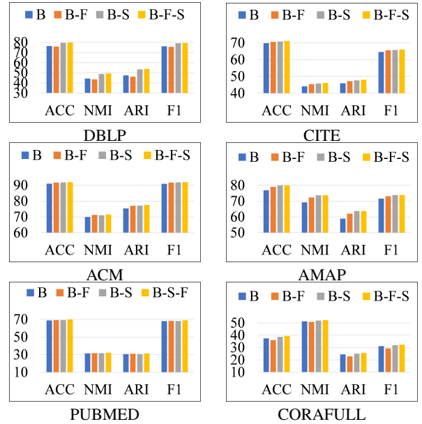
Figure 5: Ablation comparisons of dual information correlation reduction on six datasets.
