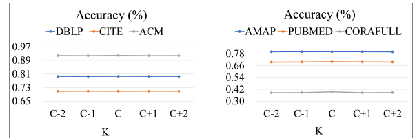
Figure 6: Clustering accuracy vs. hyper-parameter K .
