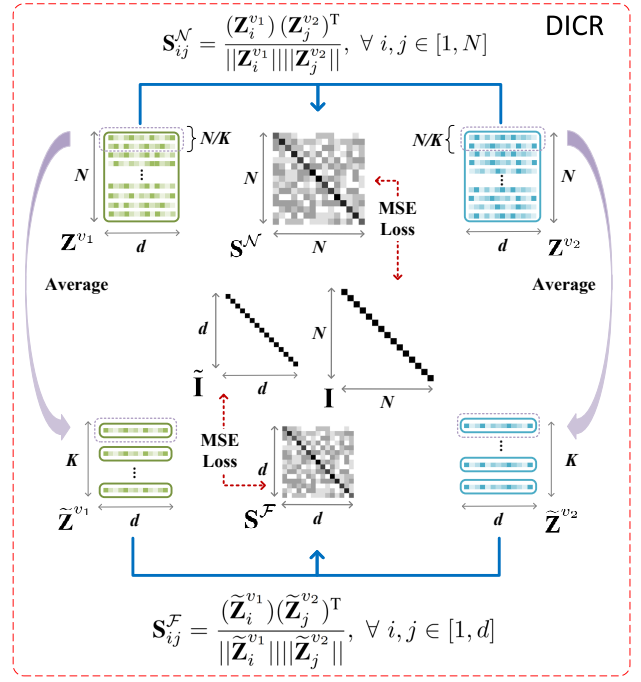
Figure 3: Illustration of Dual Information Correlation Reduction (DICR) mechanism.
